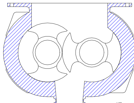
Rectangular Inlet Design
