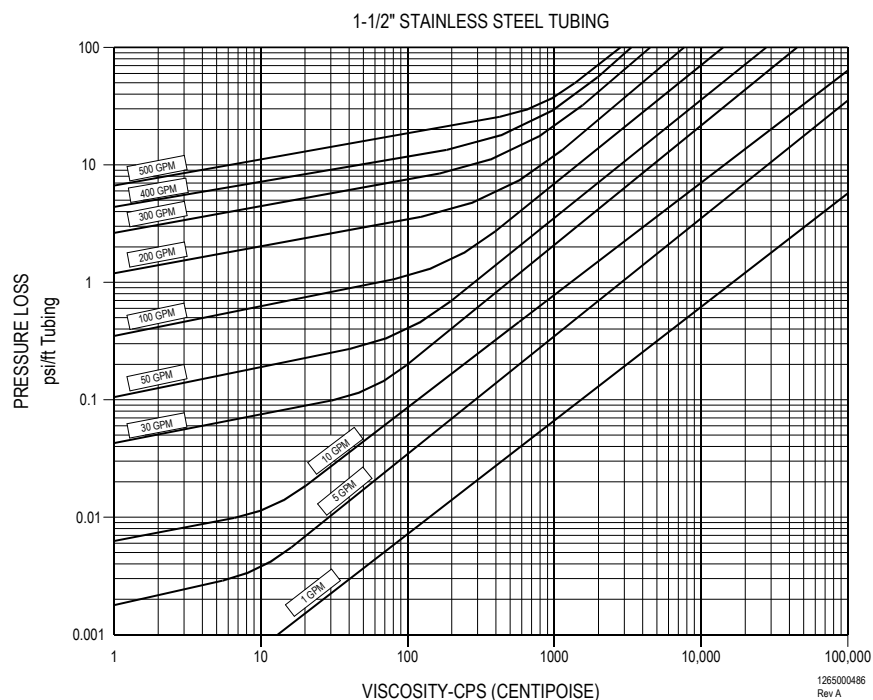
Figure 17 - Pressure loss curve - 1 ½" tubing
