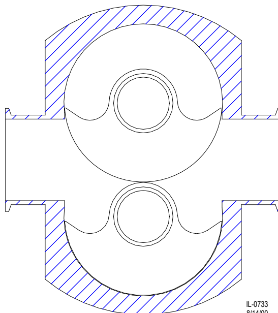
Single Lobe Rotor Design (FL II)
