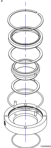
DOUBLE SEAL
