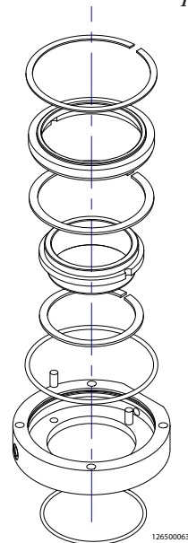
SINGLE SEAL
